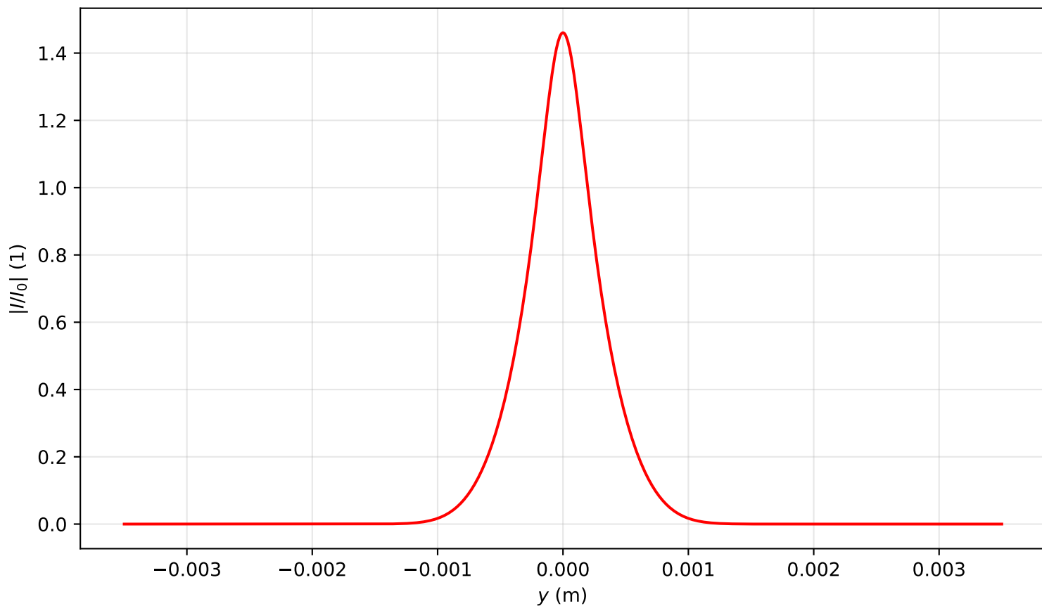
Intensity profile I(x=0, y, z=0.239)/I_0 , P_{in}=5.5P_{cr} , artificial time
